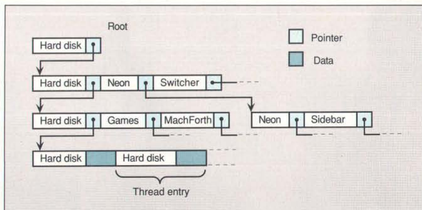
Figure 3: A portion of a Macintosh HFS catalog B*-tree. Once the system locates the root, it can rapidly locate the information for any file or directory.
